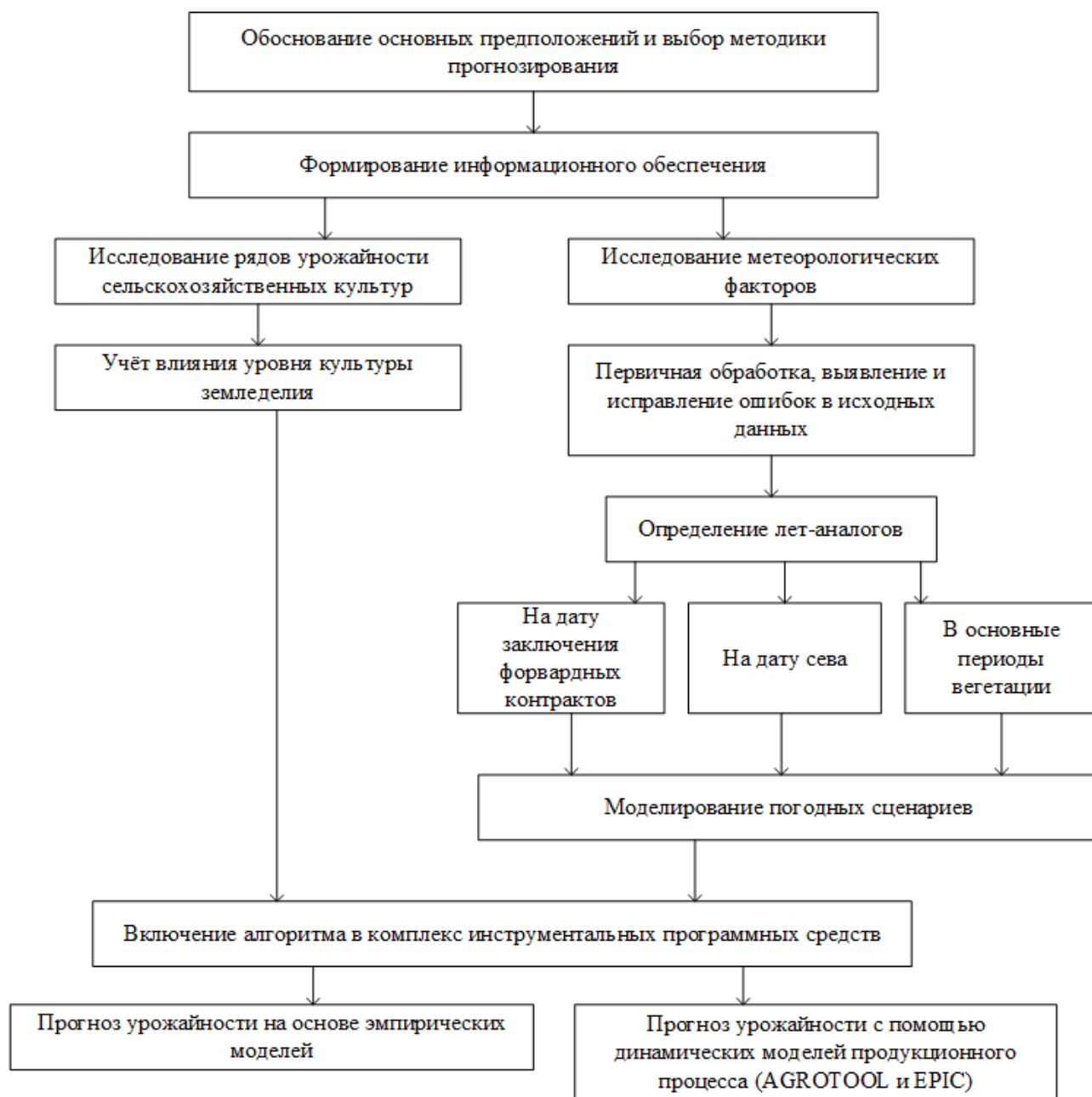
Figure 1. Block diagram of the phased yield prediction procedure.
